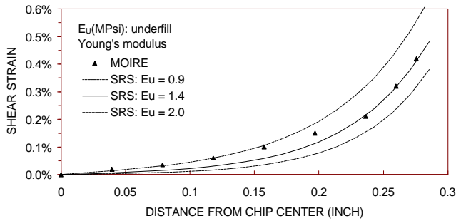
Figure 17: Shear strain distribution in underfill layer of silicon-on-ceramic test vehicle ( \Delta T = -80^\circ\text{C} ).
