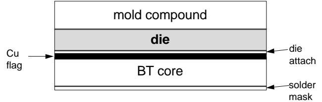
Figure 9: Schematic of multilayer construction in die area.
